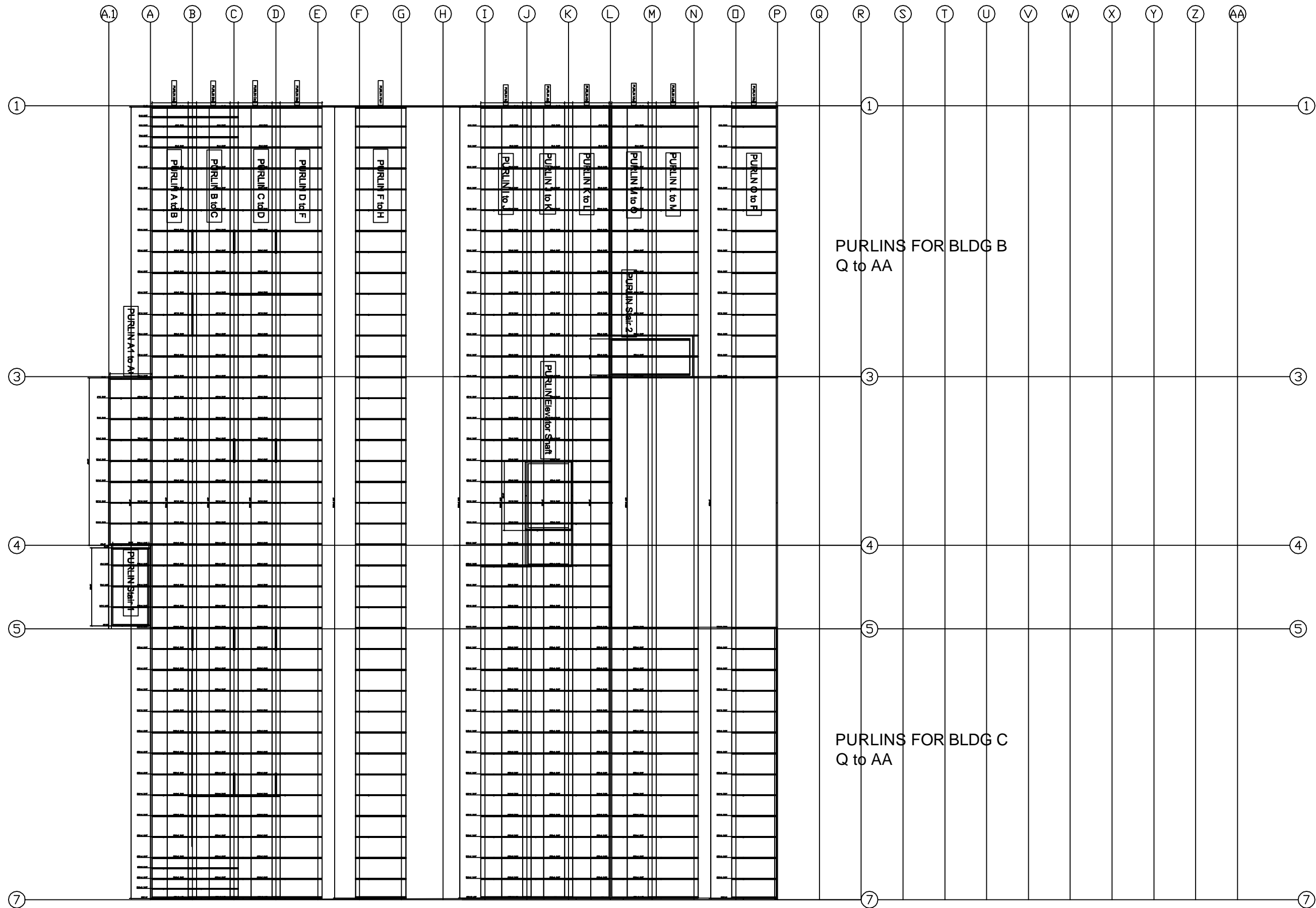
PURLIN MATERIALS KEY PLAN
